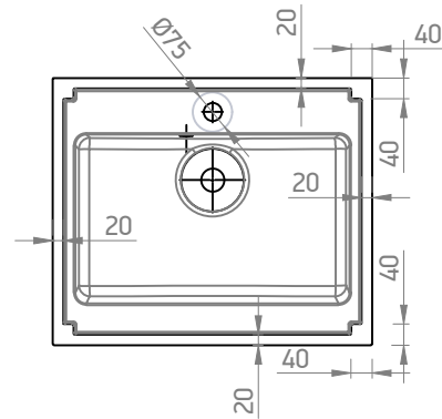
Bottom view 1:16
